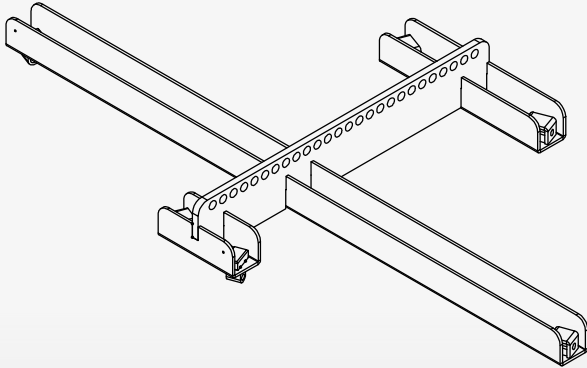
FF1-W Assembly
